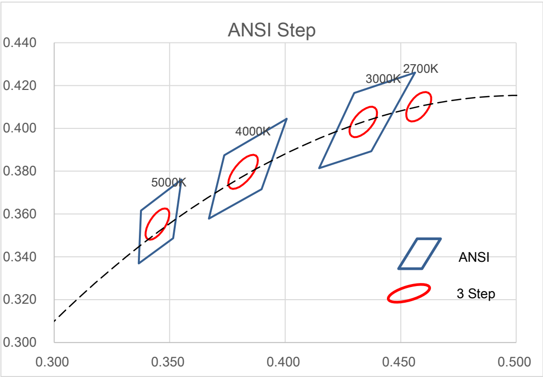
X-y chart CIE1931
