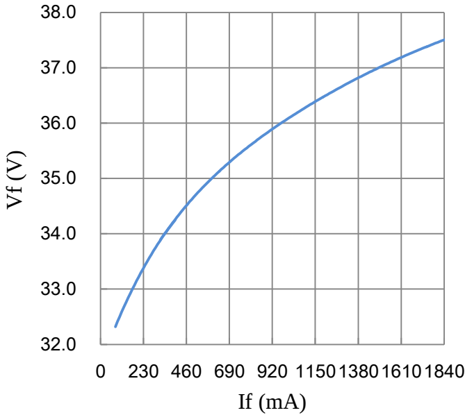
Forward Current vs. Forward Voltage ( T_c=25^\circ\text{C} )
